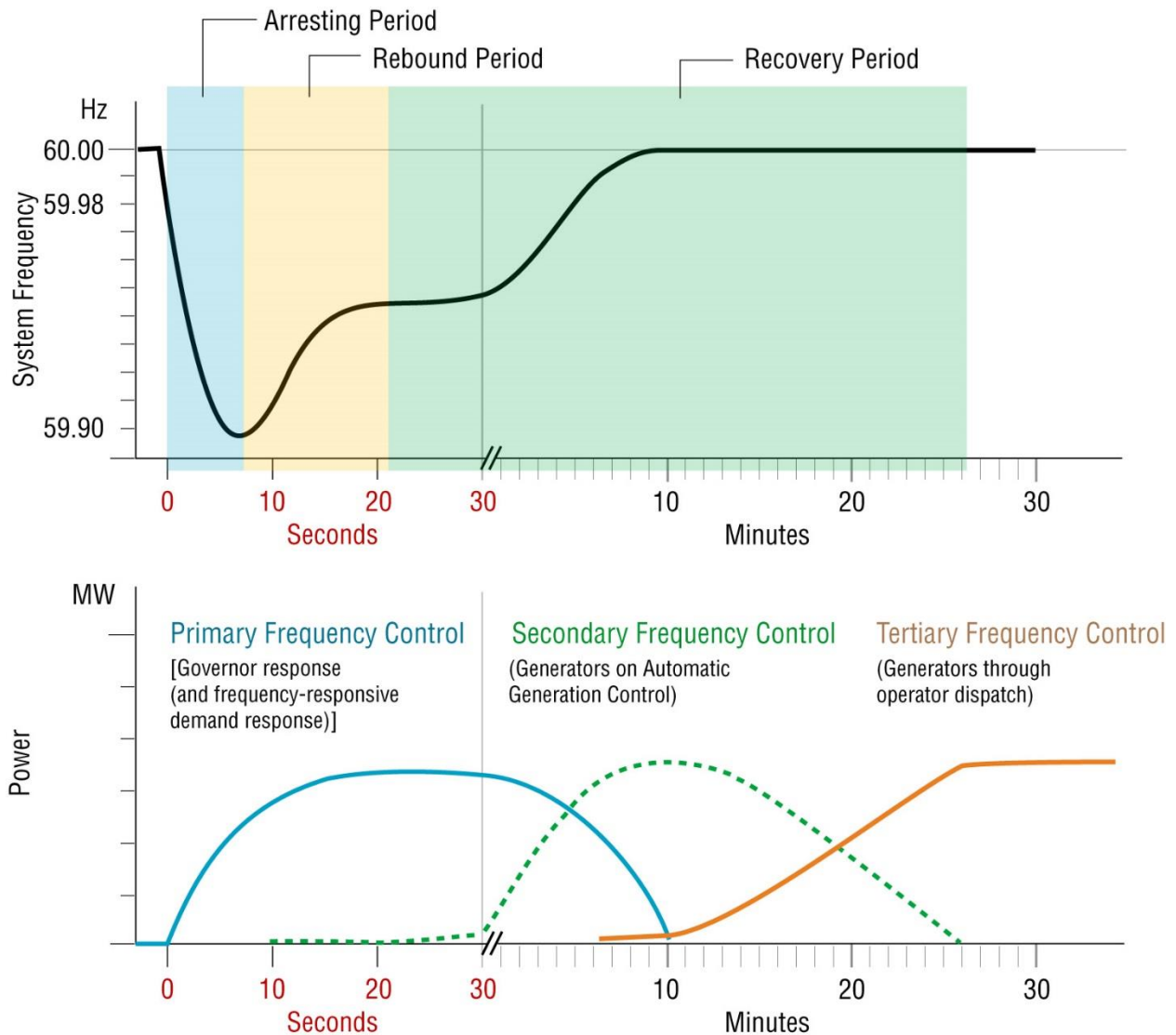
Figure 4.5. System Frequency after a Grid Event (Top) and How Frequency Control Mechanisms Work to Restore Frequency (Bottom) 243
